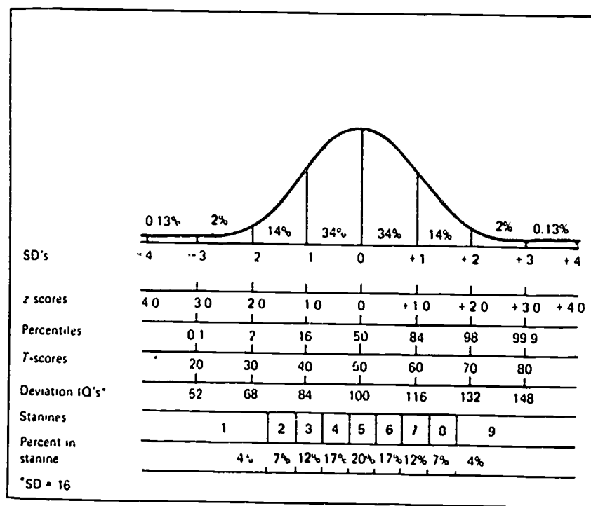
Figure 14.2 Corresponding standard scores and percentiles in a normal distribution.
