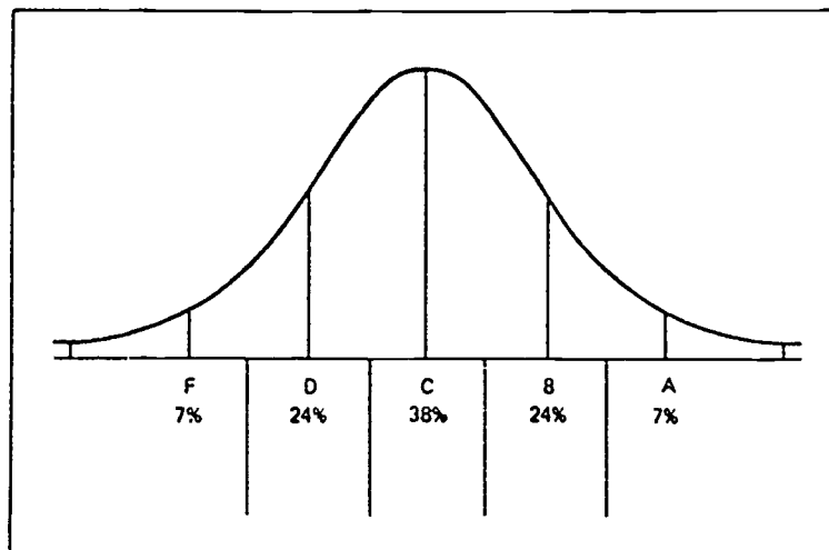
Figure 19.2 Normal curve with a typical distribution of grades. (From N. E. Gronlund, Improving Marking and Reporting in Classroom Instruction . New York: Macmillan, 1974. Used by permission.)
